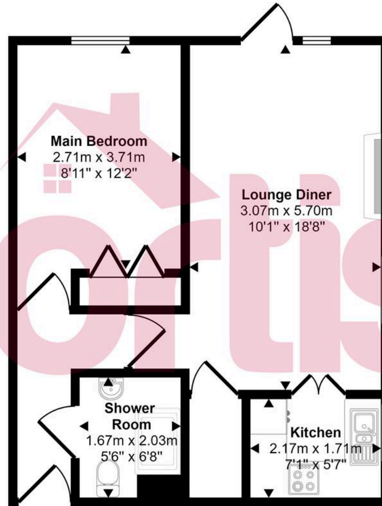
Floorplan
